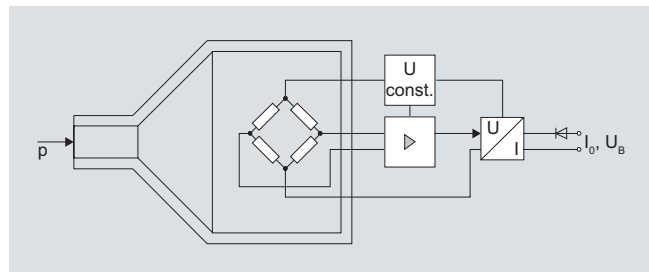
SITRANS P pressure transmitters, Z series (7MF1564-...), functional diagram
