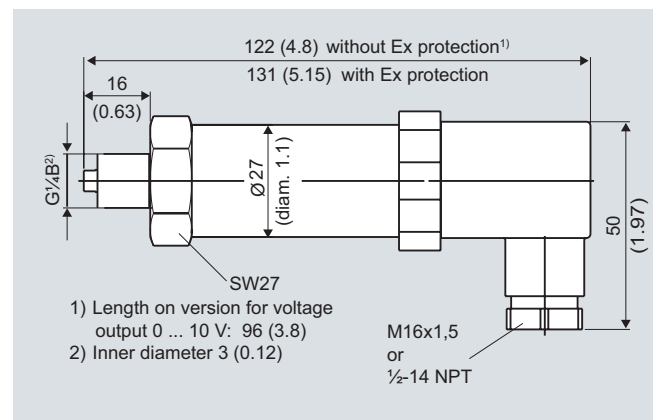
Pressure transmitter 7MF1564-... with process connection G 1/4" male, dimensions in mm (inch)
