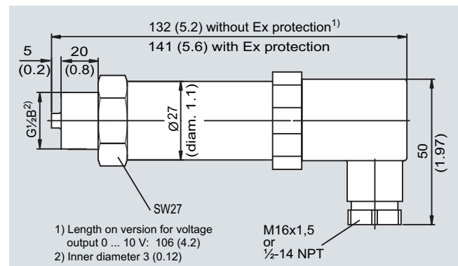
Pressure transmitter 7MF1564-... with process connection G 1/2" male, dimensions in mm (inch)
