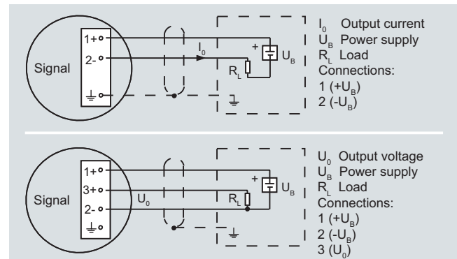
SITRANS P pressure transmitters, Z series (7MF1564-...), connection diagram, with current output (top) and voltage output (bottom)
