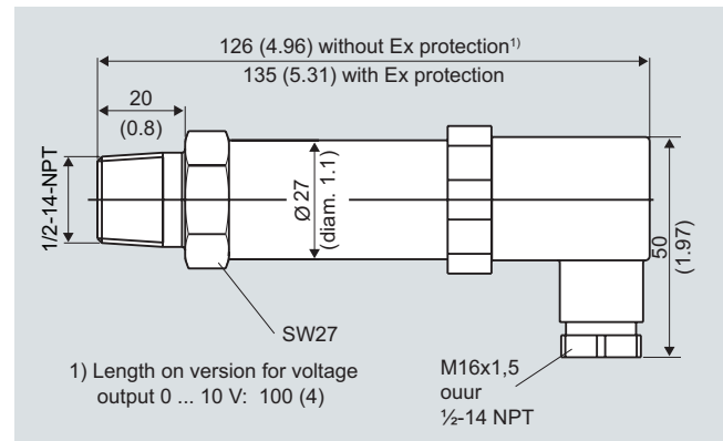
Pressure transmitter 7MF1564-... with process connection 1/2"-14 NPT male, dimensions in mm (inch)
