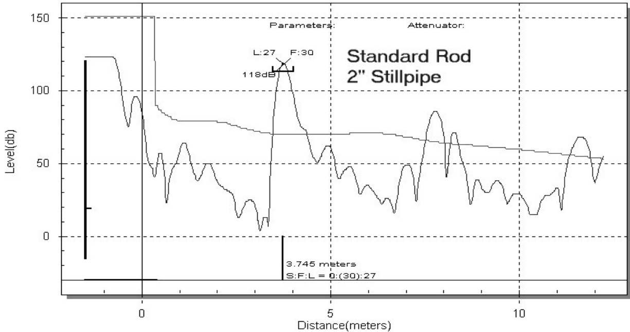
Fig. 7 Typical SITRANS LR 300 echo profile using a standard rod antenna in a 2" (50mm) still pipe.
