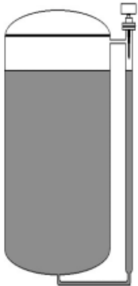
Fig. 1 SITRANS LR 300 mounted on tank equipped with side pipe.
