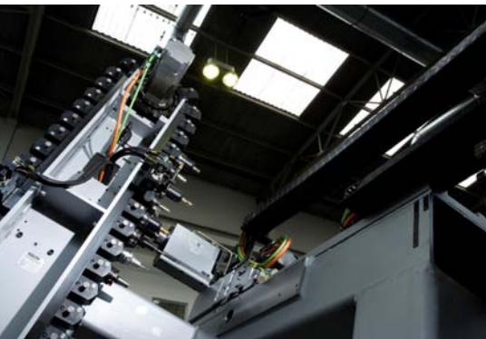
The modular concept of the tool change systems with chain magazines from ktc offers room – if required – for multiple magazines and also an additional workpiece changer.
