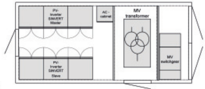
Example: 1 MW-Container with SINVERT 1000 MS TL and MV components
