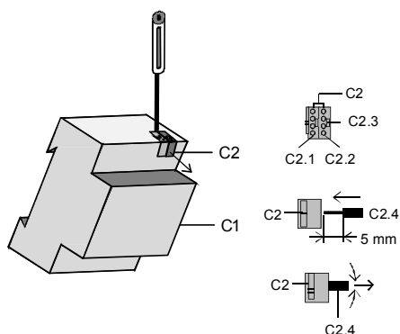
Figure 3: Connecting and removing the cable
