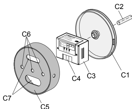
Picture 5: Installation of the brightness sensor AP 255/02
