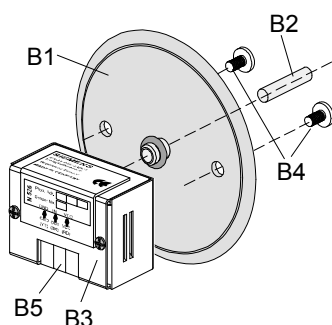
Picture 4: Installation of the brightness sensor UP 255/01
