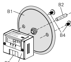
Diagram 2: Installation of the brightness sensor UP 255/01
