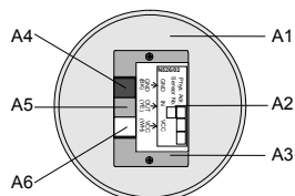
Diagram 1: Location of the operating and display elements
