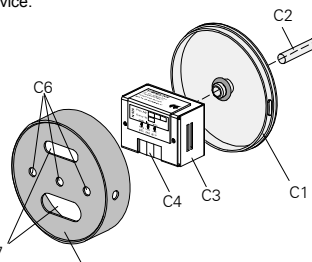
Diagram 3: Installation of the brightness sensor AP 255/02
