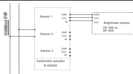
Diagram 2: Installation of the brightness sensor UP 255/01
