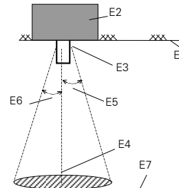
Diagram 5: Detection cone of a fibre with an even surface
