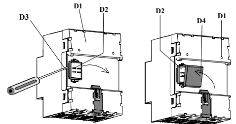
Figure 2: Covering the contact system with insulation top
