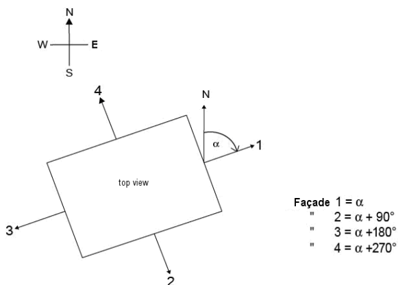
Figure 1 Façade alignment
